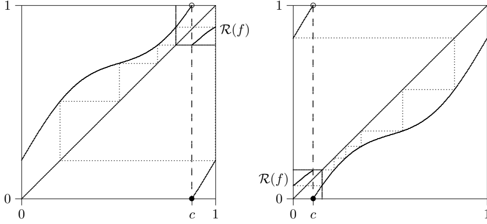
Fig. 1.2: a(f) , J_1 and the map \phi_1: J_1 \rightarrow J_1 from below when J' is to the left respectively to the right of J'' .
