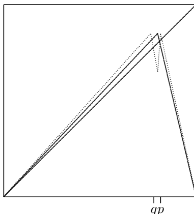
Fig. 7.1: The maps F^* and (F^*)^2 .
