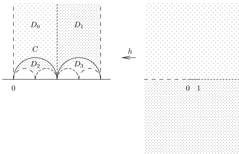
Fig. 5.3: The fundamental domain of the covering of the three punctured sphere.
